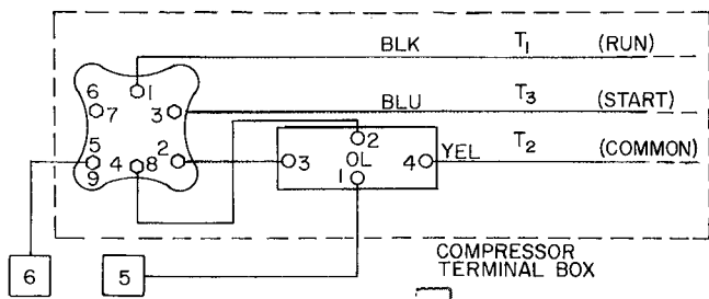
1 - PHASE A
